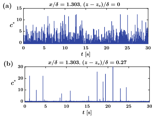
Fig. 3 First 30 s of the time-series of ethane concentration at two different wall-normal coordinates, for D/\delta = 9.55 \times 10^{-3} : a (z - z_s)/\delta = 0 , namely at the centreline; b z/\delta = 0.271 . For comparison purposes, the time-series are normalized as c^*(t) = (c(t) - \mu_c)/\sigma_c , where \mu_c and \sigma_c are the mean and standard deviation of the local time-series c(t) , respectively
