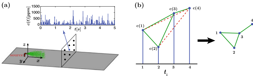
Fig. 1 a Sketch of the experimental setup. The source of passive scalar (ethane) is an L-shaped tube at z_s = 75 mm, and an example of time-series of concentration, c(t) , is also reported. The axis origin is put at the wall (i.e., z = 0 ) in correspondence with the source location. b Example of application of the visibility algorithm. A series with four temporal observations is shown as blue vertical lines (left), corresponding to the nodes of the network (right). Green solid lines represent the visibility lines between data points (see (1)) and the corresponding links in the network, while red dashed lines indicate the absence of visibility (i.e., no link)
